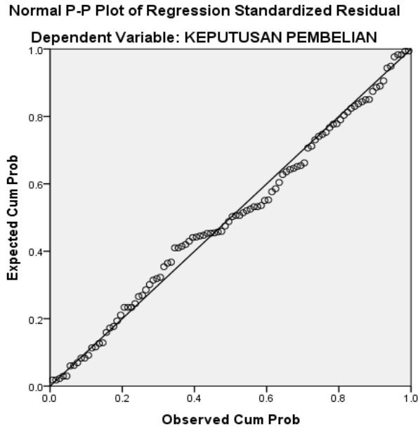
Gambar. Grafik Normality Probability Plot Sumber: Hasil Pengolahan Data SPSS 22, 2022 Gambar 4.1
