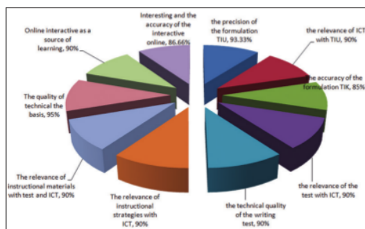
Chart 1. Second Validation Result by Instructional Design Experts [9].
