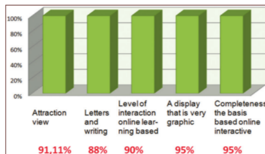
Chart 3. Media Experts' Validation Result [11].
