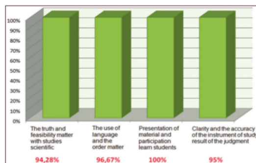
Chart 2. Chart of Subject Matter Experts' Validation Result [10].
