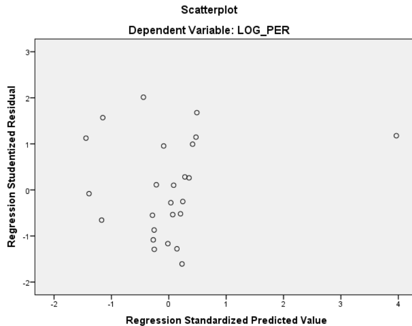
Gambar 4.1. Scatterplot
